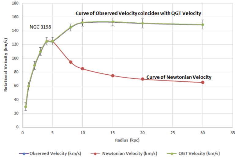
Fig. 1: Observed vs. Predicted Rotation Curve (QGT matches Observations; Newtonian fails Beyond R > 5 kpc ).
