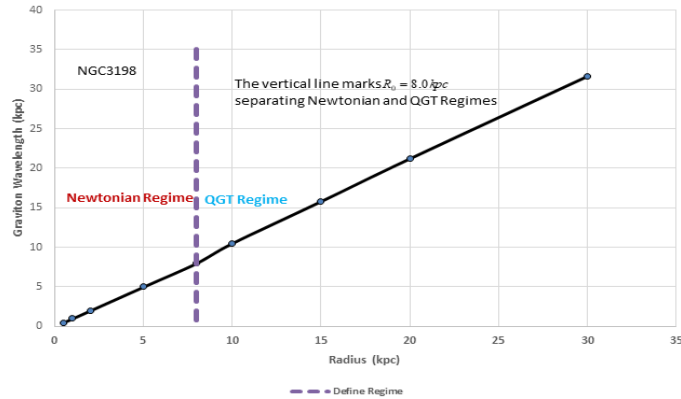
Fig. 2: Graviton Wavelength \lambda_A(R) vs. Radius. Vertical line marks R_0 = 8.0 kpc separating Newtonian and QGT regimes.
