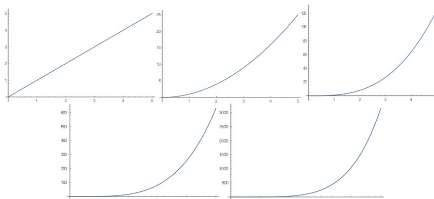
Fig. 6: Extinction Cross Section Area for Neodymium Nanorods with Effective Radius of 45 (Nm) and Various Dimension Ratios.
