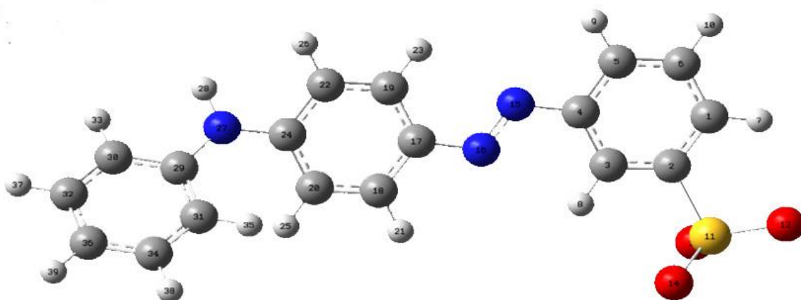
Fig. 2: Geometrically optimized structure of metanil yellow
