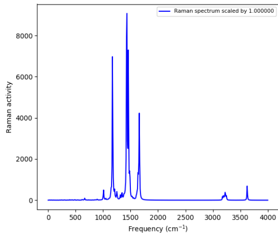
Fig. 6: Raman Spectra
