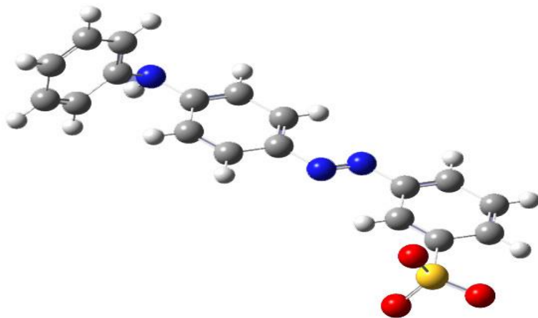
Fig. 1: Metanil Yellow
