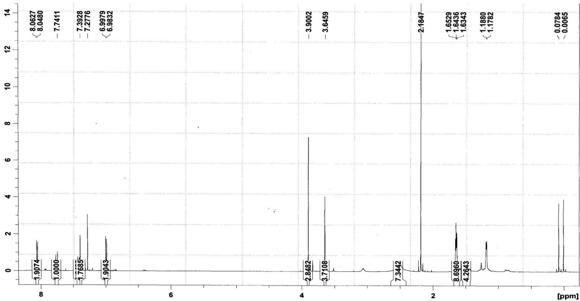
Fig 1 H NMR of 4-hydroxy-4'-methoxy-3,5-bis-piperlidinomethylchalcone (4)
