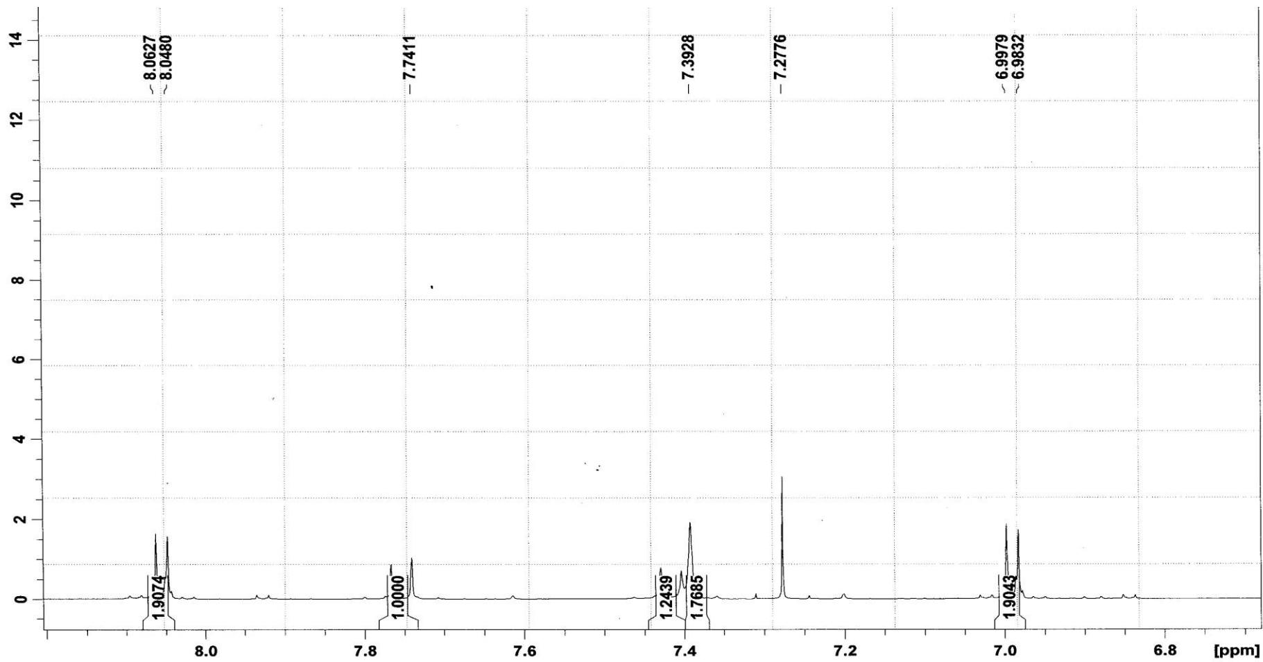
Fig ^1\text{H} NMR of 4-hydroxy-4'-methoxy-3,5-bis-piperidinomethylchalcone (4)
