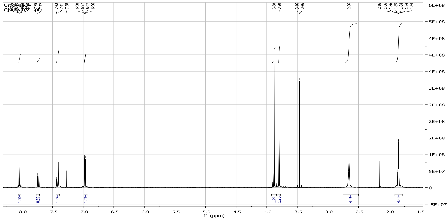
Fig 1 H-NMR spectrum of 4-hydroxy-4'-methoxy-3,5-bis-pyrrolidinomethylchalcone (3)
