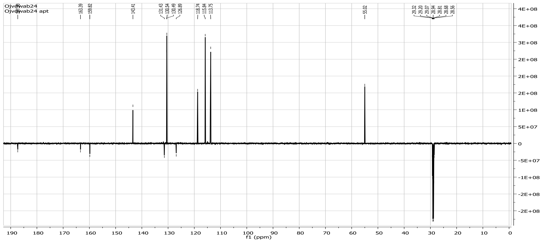
Fig Apt experiments of 4-hydroxy-4'-methoxychalcone (1)
