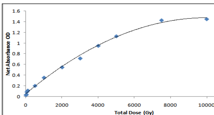
Fig.2. Plot of total dose versus net absorbance OD of the gamma irradiated PS-LMG film from 0.05 kGy to 10 kGy
