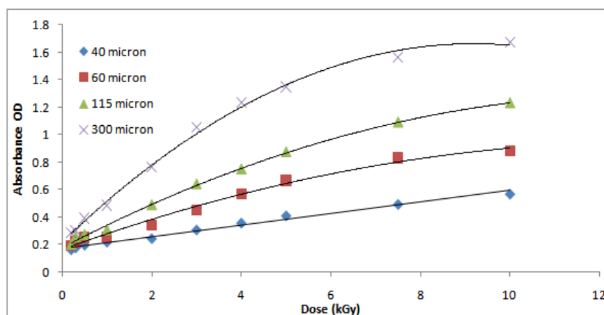
Fig. 3: Plot of Absorbance as function of increasing \gamma -doses up to 10 kGy of PS-LMG films with 40 \mu\text{m} , 60 \mu\text{m} , 115 \mu\text{m} and 300 \mu\text{m} thickness.
