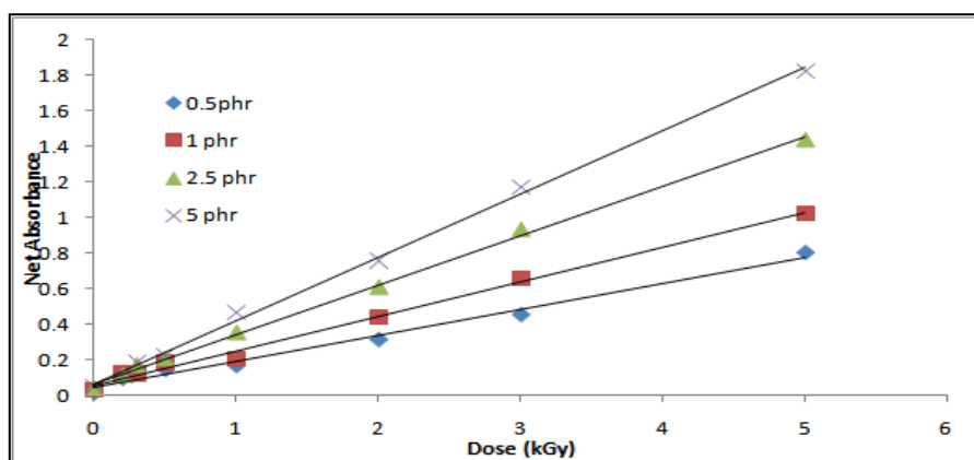
Fig. 4: Plot of Absorbance OD with increasing \gamma -doses upto 5kGy of LMG-PS films with 0.5phr, 1phr, 2.5phr and 5 Phr of LMG in the films.
