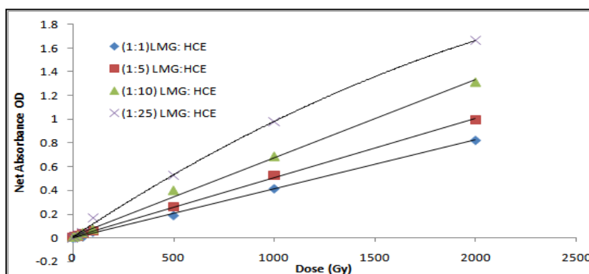
Fig. 5: Plot of Absorbance OD with increasing \gamma -doses upto 2kGy of PS-LMG films with varying ratio of LMG : Hexachloroethane ( 1:1, 1:5, 1:10 and 1:25).
