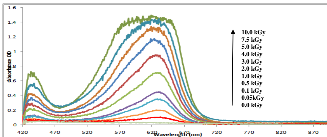
Fig. 1: Optical spectra of gamma irradiated PS-LMG film to increasing dose of radiation from 0.05 kGy to 10 kGy.
