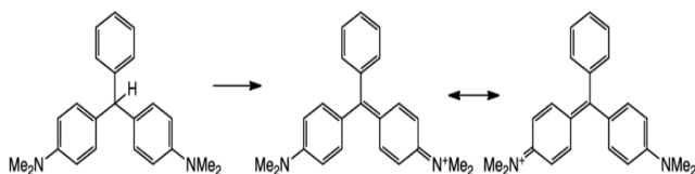
Fig. 6: Structure of LMG (Colourless) and Malachite Green (Colored).
