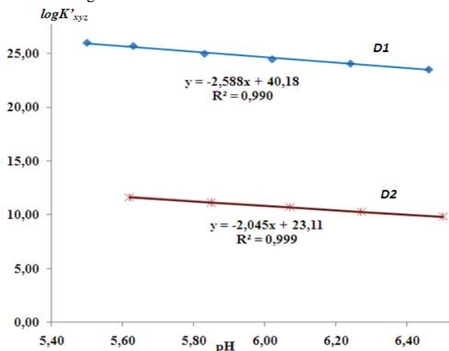
Fig. 3: The Evolution of \log K'_{xyz} at Different pH Values.
