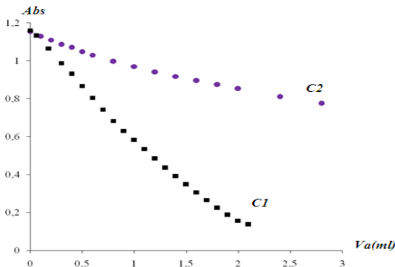
Fig. 1: Decomposition of Colored Sacrificial Complex by Addition of H 3 L and H 2 L Ions.
