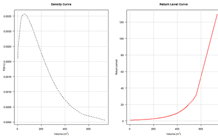
Fig. 9: Probability Density and Return Period Plot – Afon.
