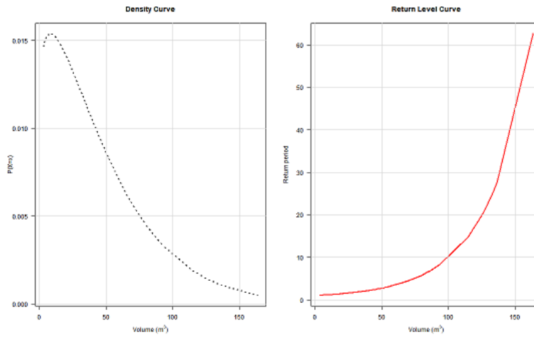
Fig. 7: Probability Density and Return Period Plot – White Afara.
