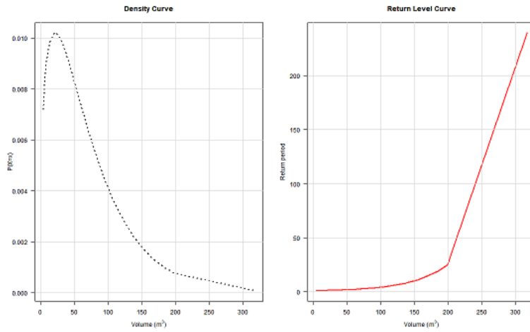
Fig. 8: Probability Density and Return Period Plot – Opepe.
