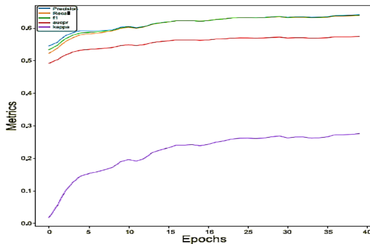
Fig. 6: CNN results
