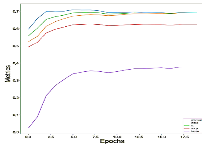
Fig. 9: CNN results
