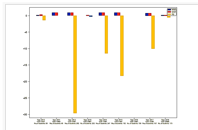
Fig. 12: CNN-LSTM results
