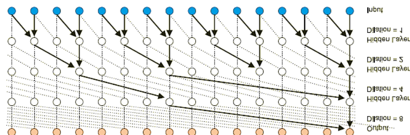
Fig. 13: Stack of Causal Dilated Conversions with l = [1, 2, 4, 8]
