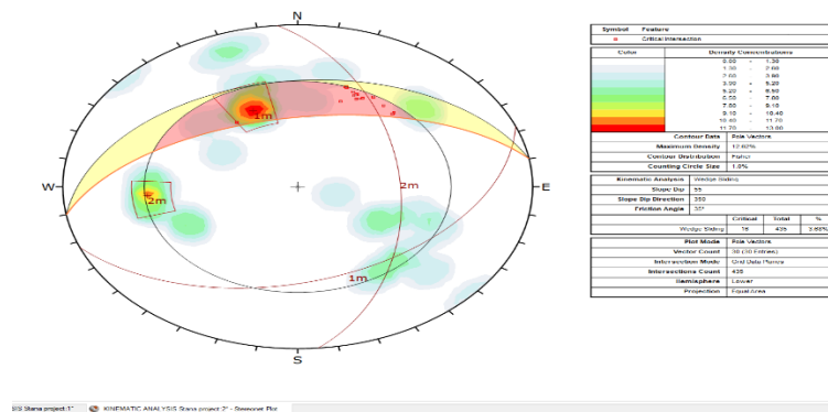
Fig. 11: Wedge Failure Criteria.
