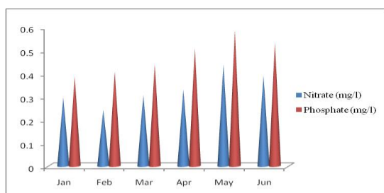
Fig. 10: Seasonal Variation of Nitrate and Phosphate (Mg/L)
