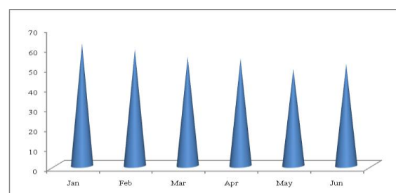
Fig. 3: Seasonal Variation of Turbidity (NTU)
