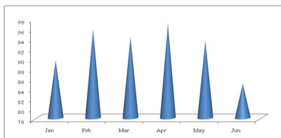
Fig. 6: Seasonal Variation of Total Alkalinity (Mg/L)
