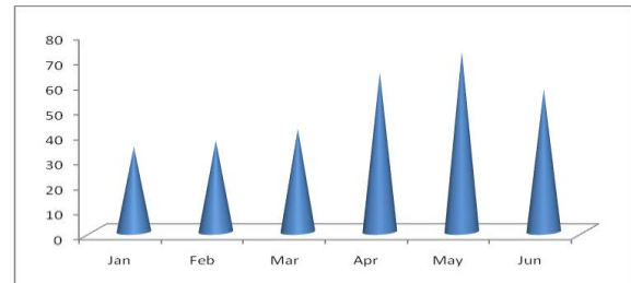
Fig. 7: Seasonal Variation of Free \text{CO}_2 (Mg/L)
