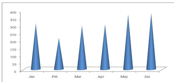
Fig. 5: Seasonal Variation of Total Dissolved Solids (Mg/L)
