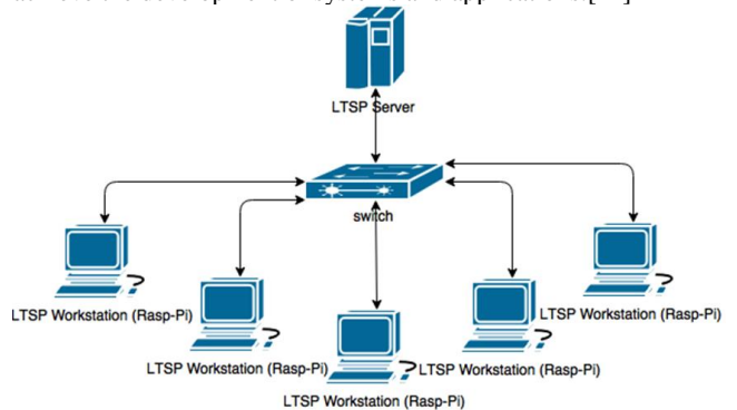
Fig. 4: Proposed Designing of Computer Thin Client with LTSP
