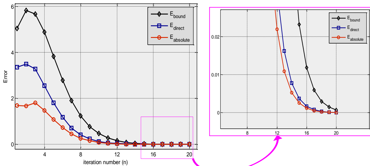
Fig. 1: Plot of Error Due To the Iteration Number ( n = 20 and h = -1.25 )
