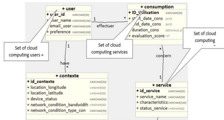
Fig. 1: Service Consumption Sub-Model.
