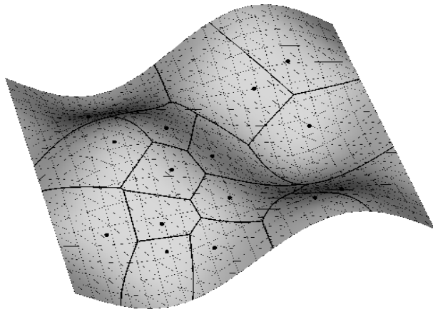
Fig. 1: The Sample Voronoi Diagram for the Wave Propagation in the Ocean.
