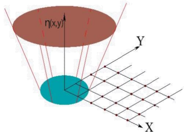
Fig. 5: Wave Front Moving Time Point Function in (X, Y) Plane.
