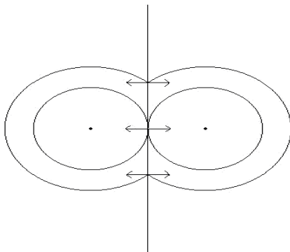
Fig. 2: The Common Axis between the Two-Wave Spread by Voronoi Diagram.
