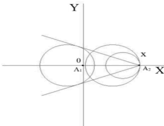
Fig. 3: The Two-Point Wave Spread by Voronoi Diagram.
