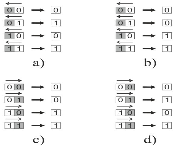
Fig. 1: Cellular Automata Conserving Mass.
