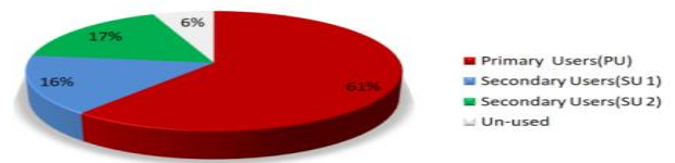
Fig. 13: Graph.
