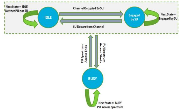
Fig. 3: Three-State-Markov-Chain-Model.
