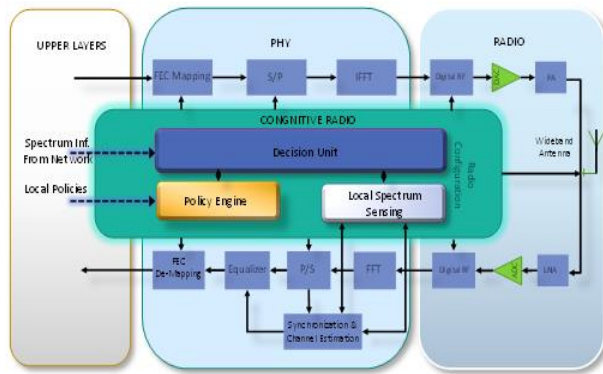
Fig. 1: Block Diagram OFDM Based Cognitive Radio.
