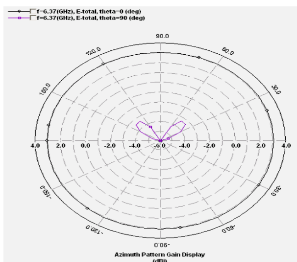
Fig. 8: Azimuth Pattern.
