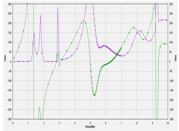
Fig. 4: Impedance Characteristics.
