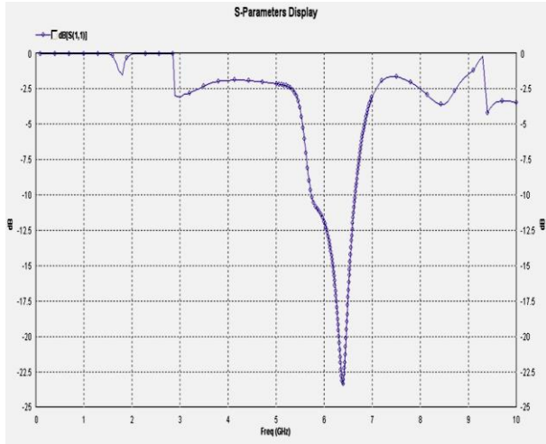
Fig. 2: Return Loss Characteristics.
