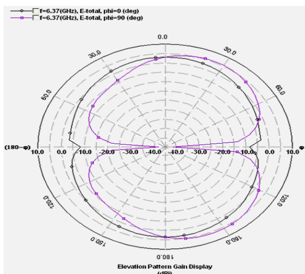
Fig. 7: Elevation Pattern.
