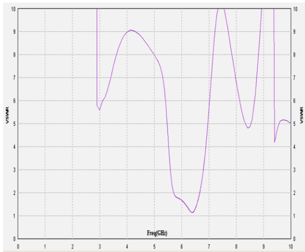
Fig. 3: VSWR Characteristics.
