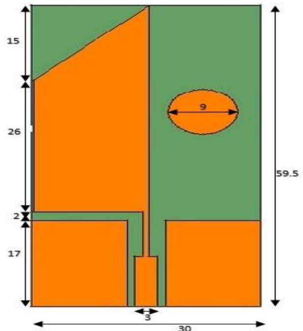
Fig. 1: Geometrical View of Proposed Antenna (Units In Mm).
