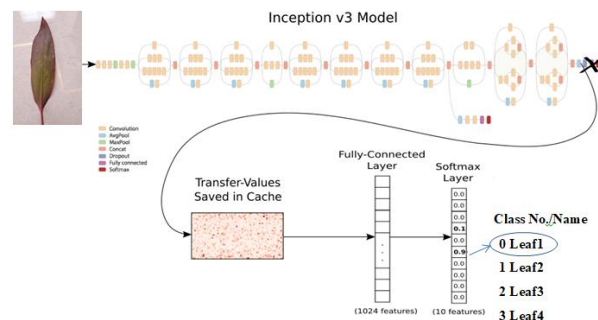
Fig 1: Training Model Using Tensorflow
