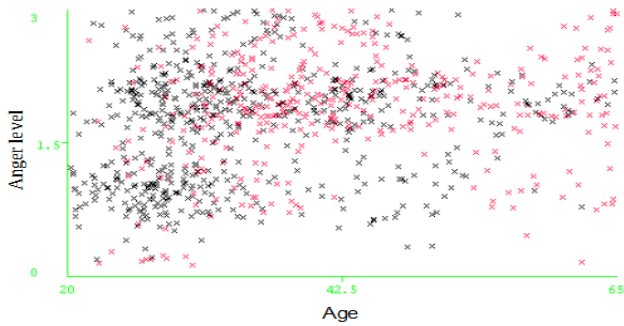
Fig. 2: HBP prediction using Age and Anger
