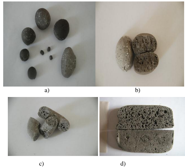
Fig. 3: Illustration of the granular thermal insulating fillers' samples, obtained in the lined molds without limitation of formation volume:
