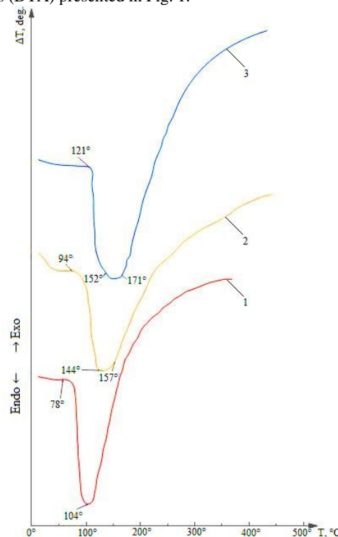
Fig. 1: DTA thermograms of sodium rare-glass composites xerogels in coordinates \Delta T - T , recorded at heating the samples in adequate conditions at different rates: curve 1 – 4 deg. / min.; curve 2 – 7 deg. / min.; curve 3 – 20 deg. / min.
