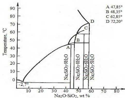
Fig. 2: Solubility in the \text{Na}_2\text{O} - \text{SiO}_2 - \text{H}_2\text{O} system
