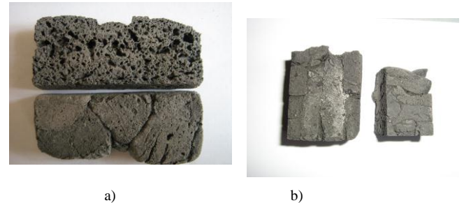
Fig. 4: Illustration of fragments of thermal insulation zones sections in complicated form structures performed by the working zone filling with fragmented elements and the subsequent heat treatment in dismantable equipment of varying complexity:
