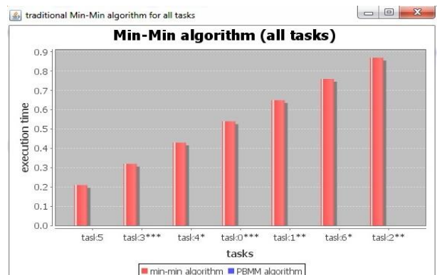
Fig. 7: Graphical Representation to Show Improvement of Min-Min Algorithm.
