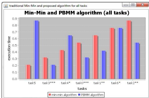
Fig. 10: Difference Performance of PBMM and Min-Min for All Tasks.
