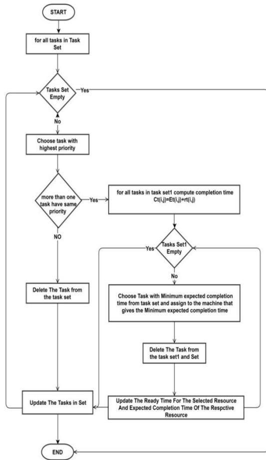
Fig. 4: Chart for PBMM Algorithm.
