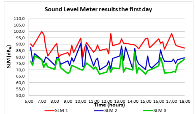
Fig. 7: The First day of Sound level meters.
