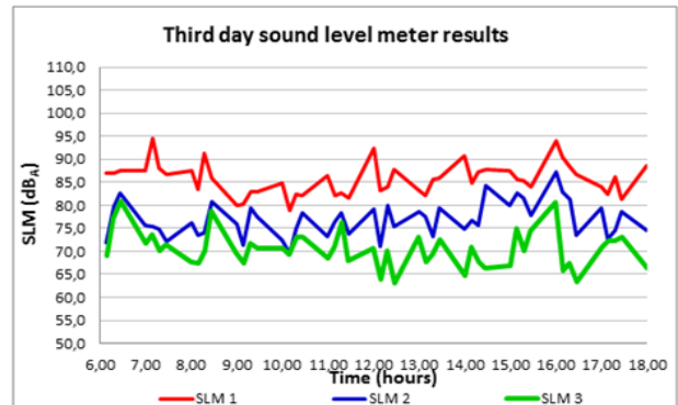
Fig. 9: The Third day of Sound level meters.
