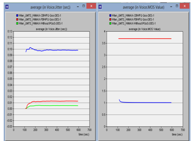
Fig. 10: Average Voice Jitter and MOS Value.
