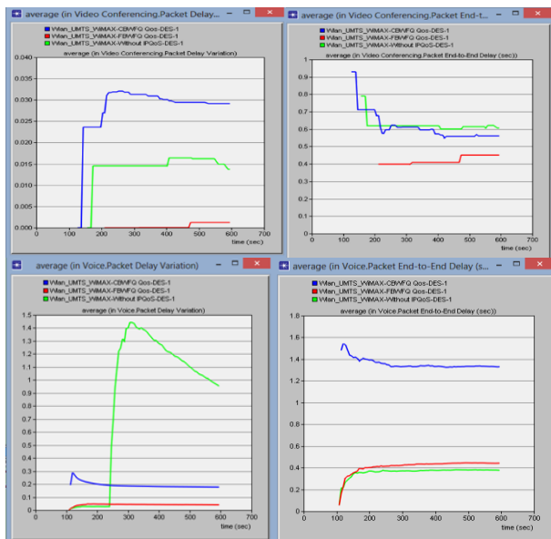
Fig. 12: Packet Delay Variation and Packet End to End Delay for Video and Voice Traffic.
