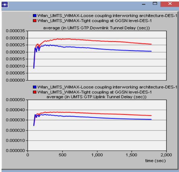
Fig. 6: UMTS Network Uplink and Downlink Tunnel Delay.
