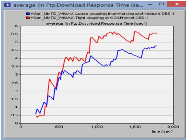
Fig. 7: FTP Download Response Time.
