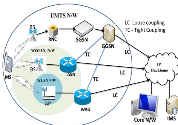
Fig. 1: Interworking Heterogeneous Networks.
