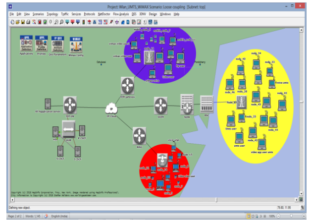
Fig. 9: WLAN-WiMAX-UMTS Interworking Architecture – Loose Coupling with IP QoS Scenario.
