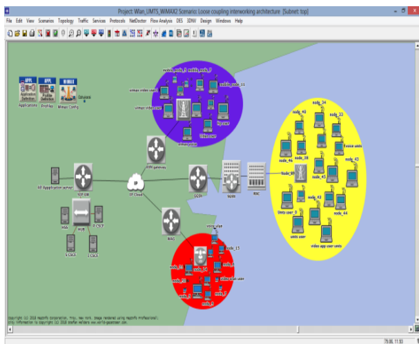
Fig. 2: WLAN-Wimax-UMTS Interworking Architecture – Loose Coupling Scenario.
