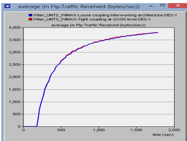
Fig. 8: FTP Traffic Received.
