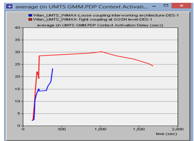
Fig. 5: UMTS Context Activation Delay.
