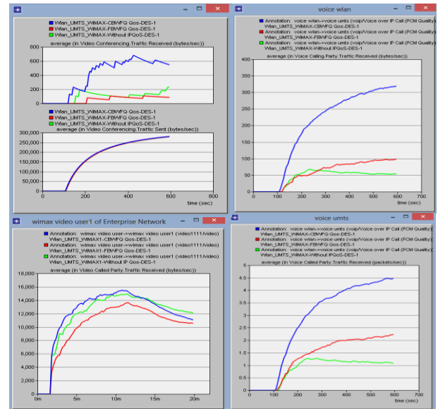
Fig. 13: Average Traffic Received for Video and Voice Traffic in WLAN, UMTS and WiMAX Networks.
