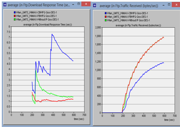
Fig. 11: Average FTP Download Response Time and Traffic Received.
