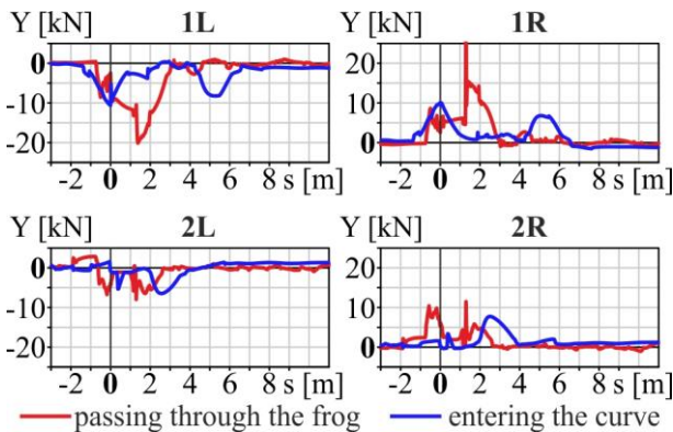
Fig. 8: Lateral forces on the individual wheels of the front bogie
