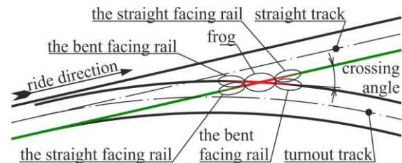
Fig. 6: Visualization of railway wheel passage through a point frog
