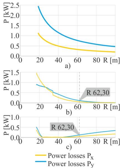
Fig. 2: Curved track passing power dissipation of the vehicle: a) without the possibility to steer the wheelsets and without additional tread, b) with the possibility to steer the wheelsets and without additional tread, c) with the possibility to steer the wheelsets and with the use of additional tread
