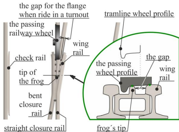
Fig. 5: Visualization of railway wheel passage through a point frog
