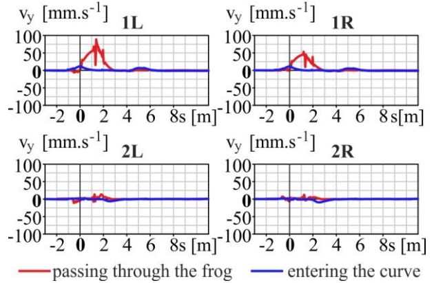
Fig. 10: Course of the lateral creep velocities on the individual wheels of the front bogie
