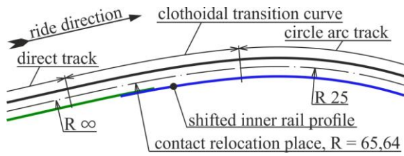
Fig. 7: Track considered in simulation when entering a small radius curve
