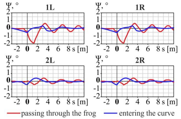
Fig. 9: Courses of angles of attack on the individual wheels of the front bogie
