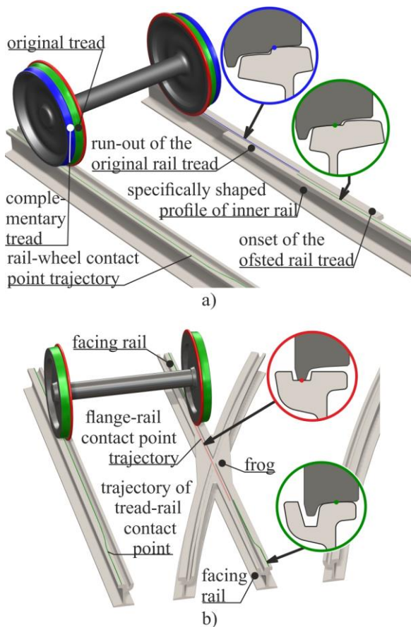
Fig. 3: Visualization of the wheelset rail-wheel contact point relocation a) on entry into a small radius curve; b) on the city lines point frog
