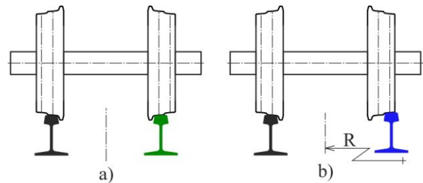
Fig. 1: Wheelset with proposed tread design a) situated in straight track, b) situated in the small radius curve
