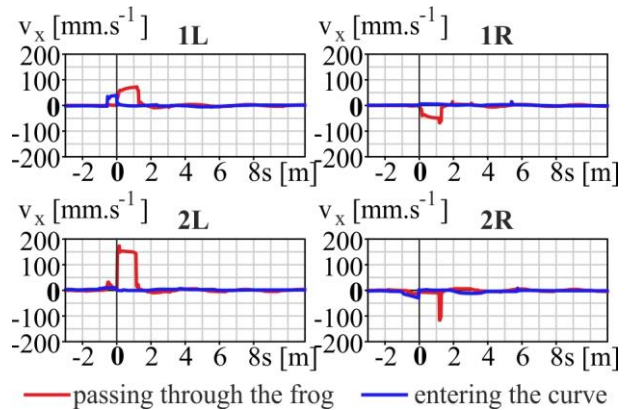
Fig. 11: Course of the longitudinal creep velocities on the individual wheels of the front bogie
