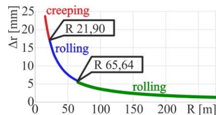
Fig. 4: Distribution of the radius of the track arc in terms of the possibility of its overcoming by rolling
