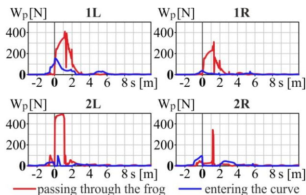
Fig. 12: Course of the sum of the wear number of contact points on the individual wheels of the front bogie
