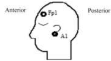
Fig. 2: Electrodes placement
