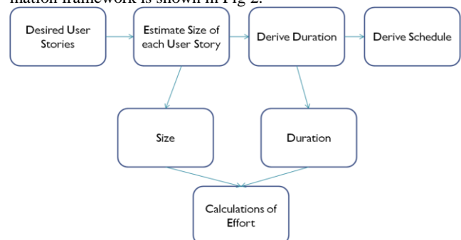
Fig 2: Generic Scrum estimation framework
