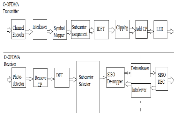
Fig. 3: Transceiver Structure of O-OFDMA for k^{th} user
