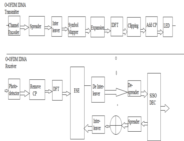
Fig. 2: Transceiver Structure of O-OFDM-IDMA for K^{\text{th}} User.
