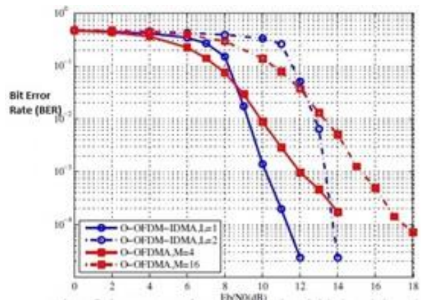
Fig. 7.:Bit Error Rate Performance in Non-Line of Sight Channels for Different L and M Values.
