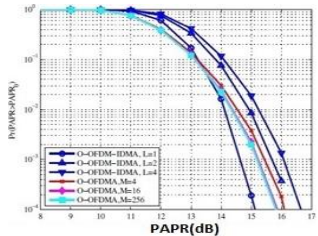
Fig. 4: Comparison of Complementary Cumulative Distribution Function Curves for Optical OFDM-IDMA and Optical OFDMA for Different L And M Values.
