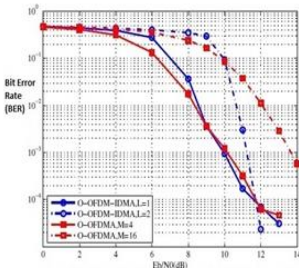
Fig. 6.:Bit Error Rate Performance in Line of Sight (LOS) Channels for Different L and M Values.
