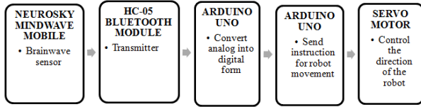
Fig.5: Block diagram of brainwave detection system [13]
