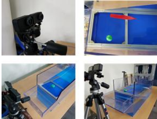
Figure 7: Experimental Environments
