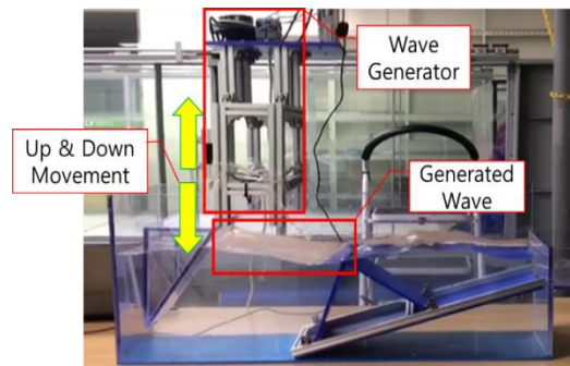
Figure 6: Constructed marine breakwater tank
