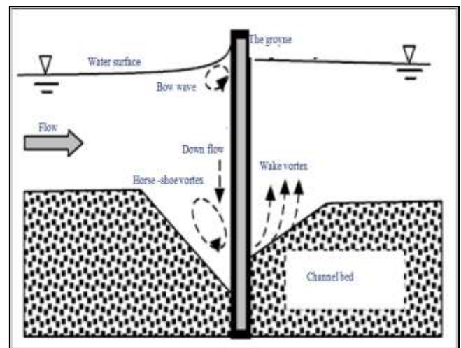
Fig. 1: Flow and local scour at the longitudinal section passing the groyne head [10]
