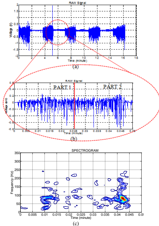
Fig.5: (a) Five repetition of the dataset, (b) one data set is separated and (c) spectrogram of the EMG signal
