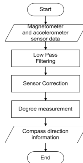
Fig. 2: Signal Processing model overview
