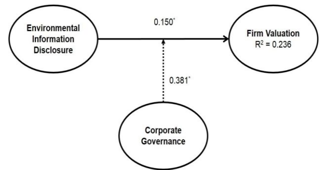
Fig. 1: PLS Results.
