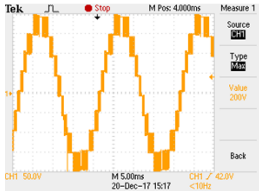
Fig. 31: 5 - Level Line Voltage at 0.8 MI.
