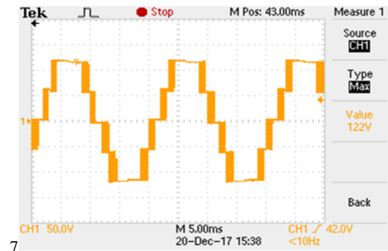
Fig. 35: 3 - Level Line - Line Voltage at 1.2 MI.
