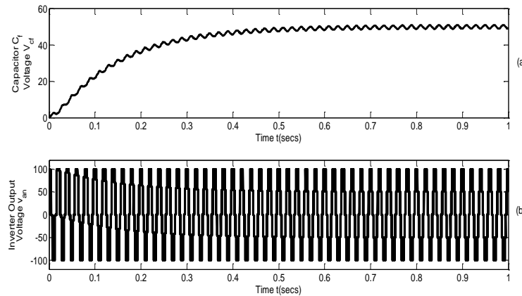
Fig. 18: (A) Capacitor voltage V_{cf} (B) Output load voltage V_{an} under self-capacitor voltage balance for the Type B hybrid multi-level inverter of Figure 17 with per cycle switch state sequence of 1 \rightarrow 2 \rightarrow 4||5 \rightarrow 6 \rightarrow 8 & C_f = 7500 \mu\text{F} , V_{dc} = 200 \text{ V} , F_c = 1.05 \text{ kHz} , F = 50 \text{ Hz} , M = 0.8 , Z_L = (5+20j) \Omega .
