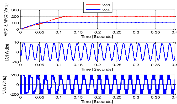
Fig. 5: (A) Capacitor voltages V_{c1} and V_{c2} . (B) Inverter output current ( I_{an} ); (C) Inverter output Voltage ( V_{an} ) under a balanced capacitor voltage control for Type A hybrid five-level inverter V_{dc} = 400 V, F_c = 5 kHz, F_s = 50 Hz, M = 0.8 , with zero pre-charged capacitor voltage.
