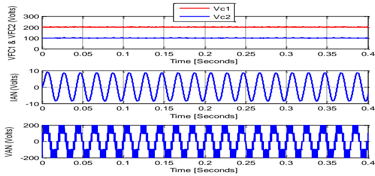
Fig. 6: (A) Capacitor Voltages V_{c1} and V_{c2} . (B) Inverter Output Current ( I_{an} ). (C) Inverter Output Voltage ( V_{an} ) Under A Balanced Capacitor Voltage Control For Type A Hybrid Five-Level Inverter V_{dc} = 400 V, F_C = 5 kHz, F_s = 50 Hz, M = 0.8 , with 100 V And 200 V Pre-Charged Capacitor Voltage.
