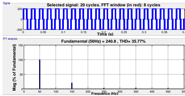
Fig. 14: Three Level Phase Voltage ( V_{an} ) With A Bypassed H-Bridge And Full Power.
