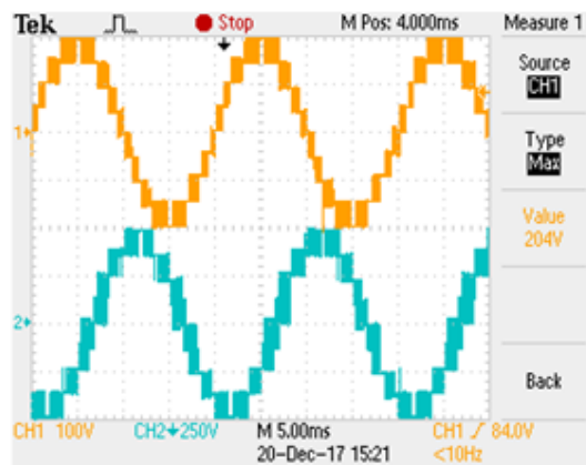
Fig. 32: 5 - Level Line - Line Voltage at 0.8 MI.
