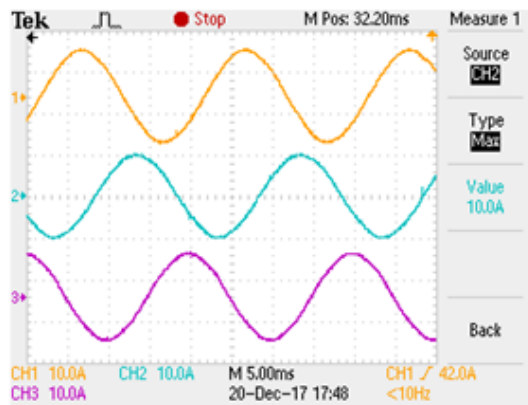
Fig. 33: 5 - Level Phase Currents at 0.8 MI.
