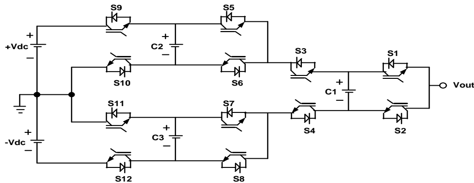
Fig. 16: Circuit Diagram of Five-Level ANPC.
