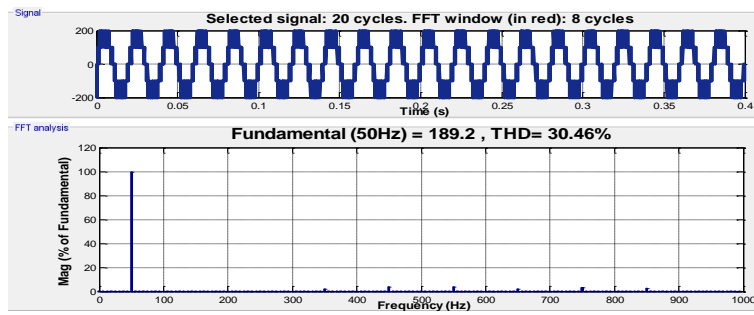
Fig. 7: Phase A Output Voltage ( V_{an} ) with A Balanced Capacitor Voltage for Type A Hybrid Multi-Level Inverter of Figure 1. V_{dc} = 400 V, F_C = 5 kHz, F_s = 50 Hz, M = 0.8 , Z_L = (8+6j) \Omega .
