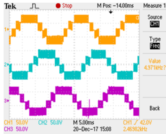
Fig. 30: Five Level Phase Voltage at 0.8 MI.
