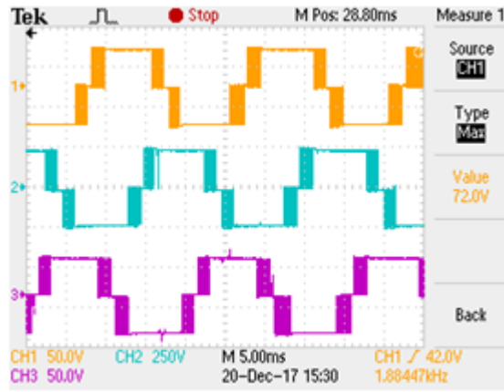
Fig. 34: 3 - Level Phase Voltage at 1.2 MI.
