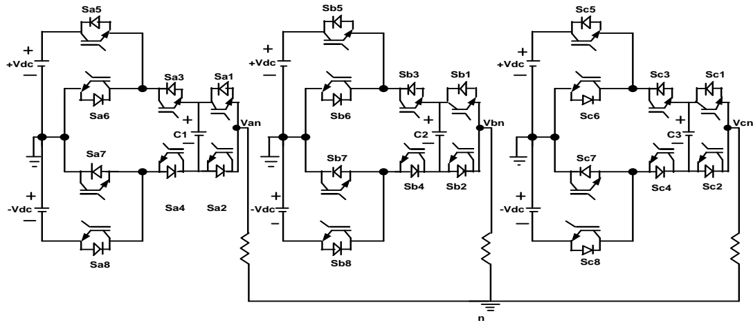
Fig. 17: Modified Circuit Diagram of Five-Level ANPC.
