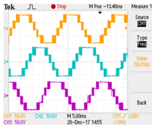
Fig. 29: Five Level Phase Voltage at 1.2 MI.
