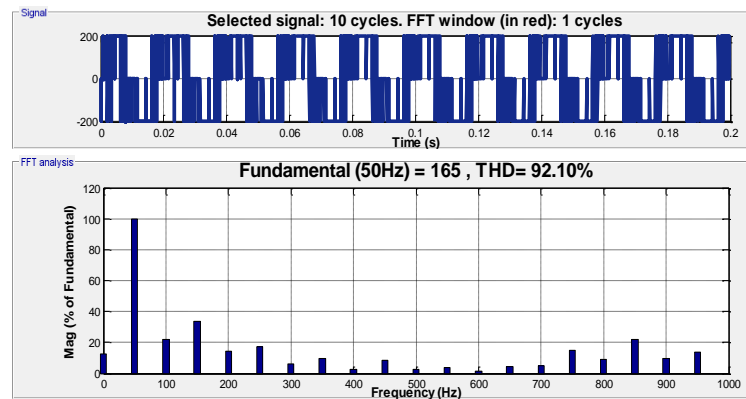
Fig. 25: Phase Voltage V_{an} of five-level ANPC inverter of Figure 17 with A Shorted Capacitor V_{dc} = 400V , F_c = 5 \text{ kHz} , F = 50\text{Hz} , M = 0.8 , Z_L = (8+6j) \Omega .
