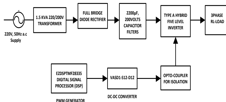
Fig. 27: Block Diagram of the Dc Power Supply Stage.
