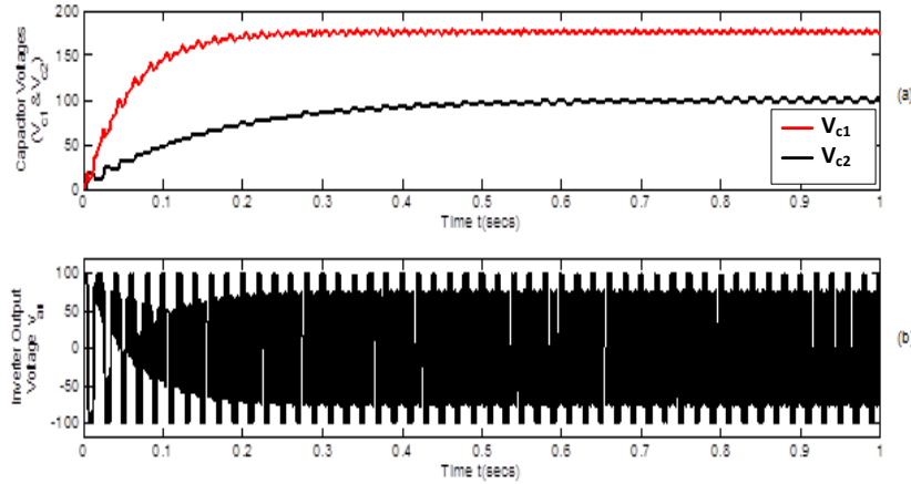
Fig. 3: (A) Capacitor Voltages V_{c1} and V_{c2} . (B) Inverter Output Voltage ( V_{an} ) for An Unbalanced Condition of Type A Hybrid Five-Level Inverter V_{dc} = 200 V, F_c = 5 kHz, F_s = 50 Hz, M = 0.8 .
