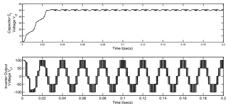
Fig. 20: (A) Capacitor Voltage V_{cf} (B) Output Load Voltage V_{an} Under Natural Capacitor Voltage Balance for the Type B Hybrid Multi-Level Inverter of Figure 17 with Per Cycle Switch State Sequence Of 1 \rightarrow 2 \rightarrow 3 \rightarrow 4 \rightarrow 5 \rightarrow 6 \rightarrow 7 \rightarrow 8 And C_f = 1500 \mu\text{F} , V_{dc} = 200 \text{ V} , F_c = 1.05 \text{ KHz} , F = 50\text{Hz} , M = 0.8 , Z_L = (8+6j) \Omega .
