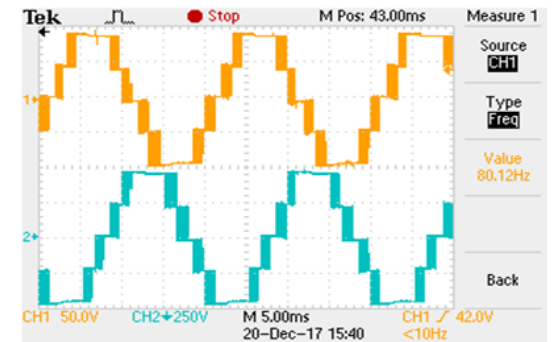
Fig. 36: 3 - Level Line - Line Voltage at 1.2 MI.
