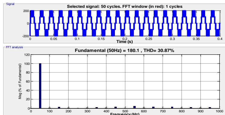
Fig. 23: Phase Voltage V_{an} of five-level ANPC inverter of Figure 17 under natural capacitor voltage balancing operation. V_{dc} = 400V , F_C = 5 kHz , F = 50 Hz , M = 0.8 , Z_L = (8+6j) \Omega .
