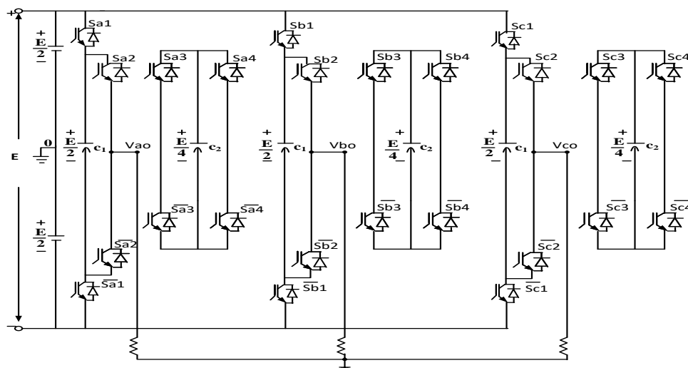
Fig. 2: Diagram of Type A Hybrid Five-Level Inverter with A Bypassed H-Bridge.
