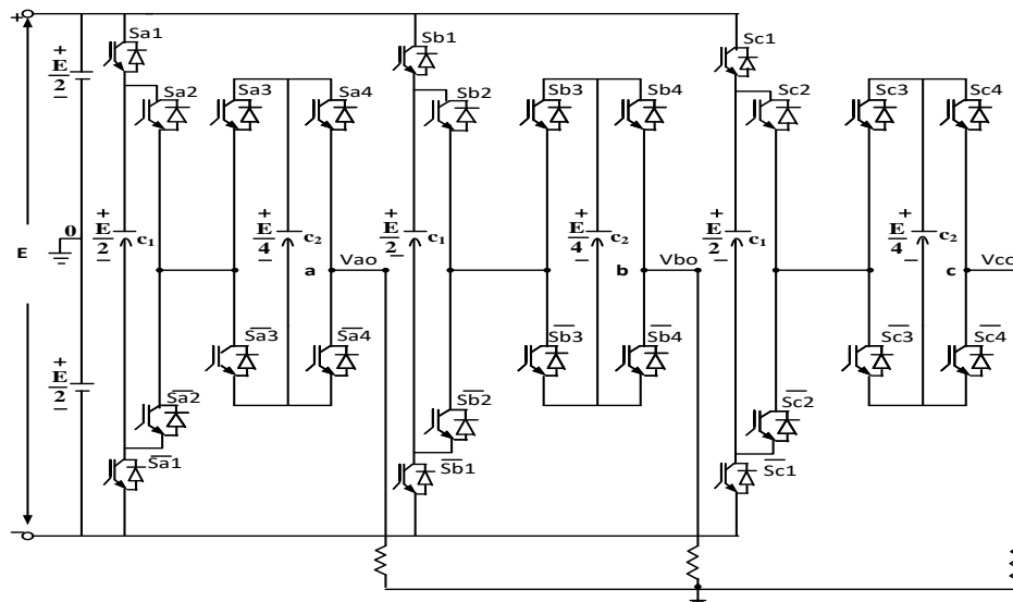
Fig. 1: Diagram of Type A Hybrid Five-Level Inverter with An Un-Bypassed H-Bridge.
