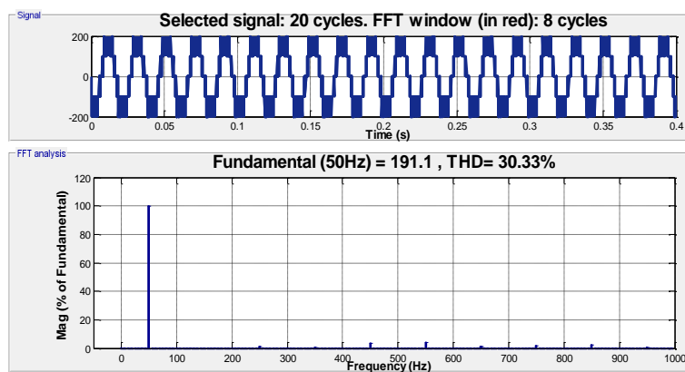
Fig. 9: Phase C Output Voltage ( V_{cn} ) with a balanced capacitor voltage for Type A hybrid multi-level inverter of Figure 1. V_{dc} = 400 V, F_C = 5 kHz, F_s = 50 Hz, M = 0.8 , Z_L = (8+6j) \Omega
