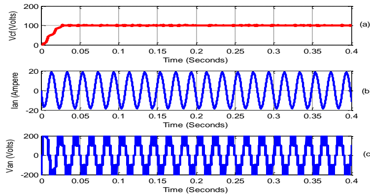
Fig. 21: (A) Capacitor voltage V_{cf} (B) Output Phase Current I_{an} (C) Output Phase Voltage V_{an} under natural capacitor voltage balancing operation for the five level ANPC inverter of Figure 17 with per cycle switch state sequence of 1 \rightarrow 2 \rightarrow 3 \rightarrow 4 \rightarrow 5 \rightarrow 6 \rightarrow 7 \rightarrow 8 and C_f = 1500\mu F , V_{dc} = 400 V , F_C = 5 kHz , F = 50 Hz , M = 0.8 , Z_L = (8+6j) \Omega with zero pre-charged capacitor voltage.
