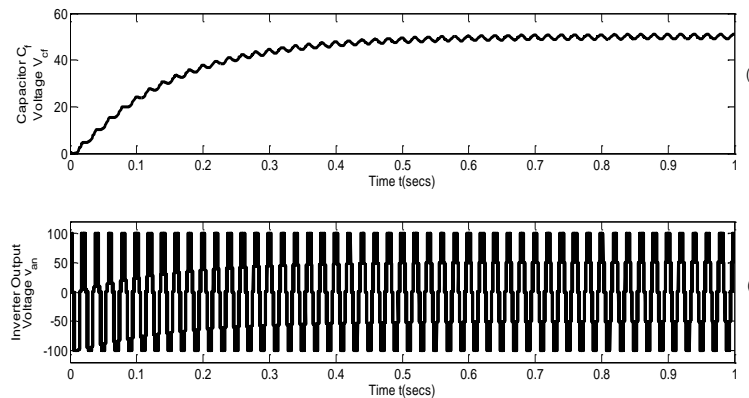
Fig. 19: (A) Capacitor voltage V_{cf} (B) Output load voltage V_{an} under self-capacitor voltage balance for the Type B hybrid multi-level inverter of Figure 17 with per cycle switch state sequence of 1 \rightarrow 3 \rightarrow 4||5 \rightarrow 7 \rightarrow 8 & C_f = 7500 \mu\text{F} , V_{dc} = 200 \text{ V} , F_c = 1.05 \text{ kHz} , F = 50 \text{ Hz} , M = 0.8 , Z_L = (5+20j) \Omega .
