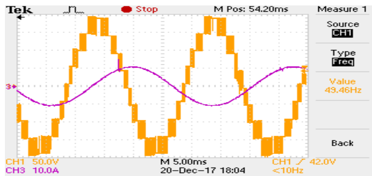
Fig. 37: An Interfaced Five Level Line Voltage and Current at 0.8 MI.
