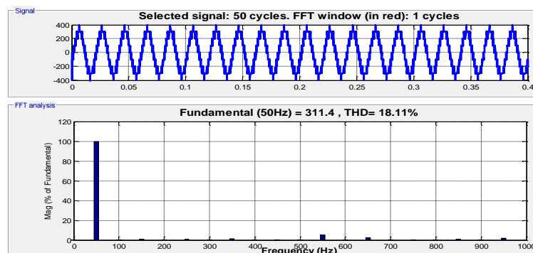
Fig. 24: Lines AB Voltage V_{AB} of five-level ANPC inverter of Figure 17 under natural capacitor voltage balancing operation. V_{dc} = 400V , F_C = 5 kHz , F = 50Hz , M = 0.8 , Z_L = (8+6j) \Omega .
