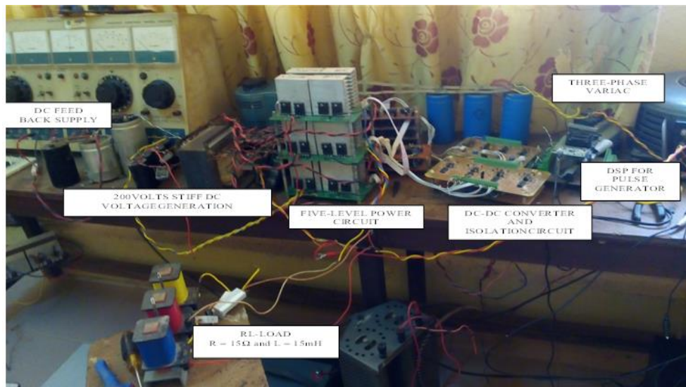
Fig. 38: Laboratory Set Up of the RL-Load with the Power Circuit and DSP.
