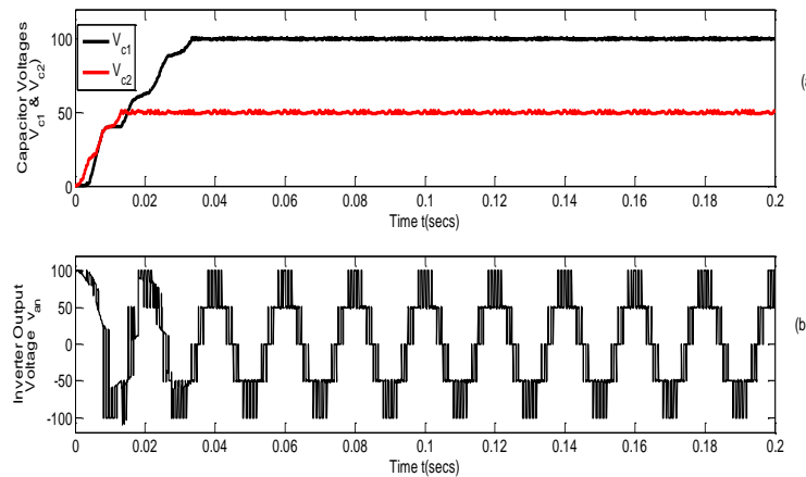
Fig. 4: (A) Capacitor Voltages V_{c1} and V_{c2} . (B) Inverter Output Voltage ( V_{an} ) for a balanced Condition of Type A hybrid five-level inverter, F_c = 5 kHz, F_s = 50 Hz, M = 0.8 .
