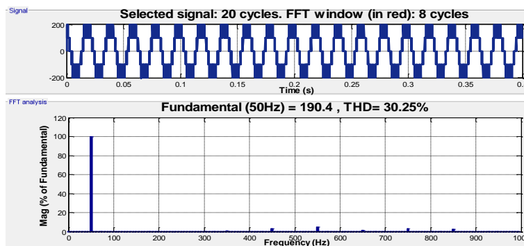
Fig. 8: Phase B Output Voltage ( V_{bn} ) with A Balanced Capacitor Voltage for Type A Hybrid Multi-Level Inverter of Figure 1. V_{dc} = 400 V, F_C = 5 kHz, F_s = 50 Hz, M = 0.8 , Z_L = (8+6j) \Omega .
