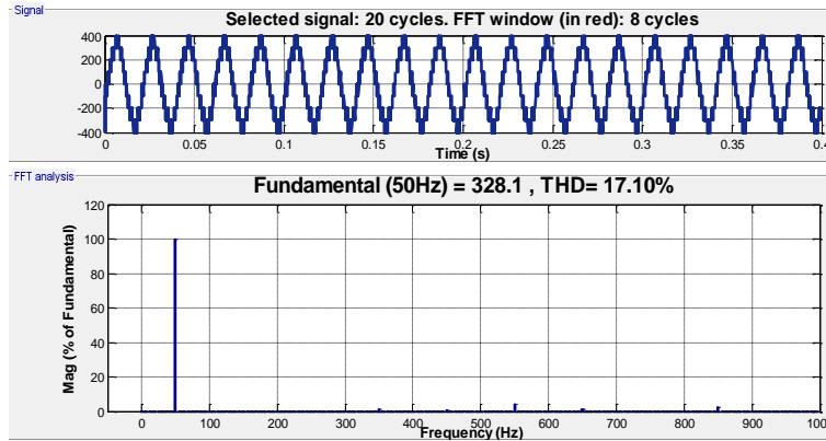
Fig. 10: Lines AB output Voltage ( V_{AB} ) with a balanced capacitor voltage for Type A hybrid multi-level inverter of Figure 1. V_{dc} = 400 V, F_C = 5 kHz, F_s = 50 Hz, M = 0.8 , Z_L = (8+6j) \Omega
