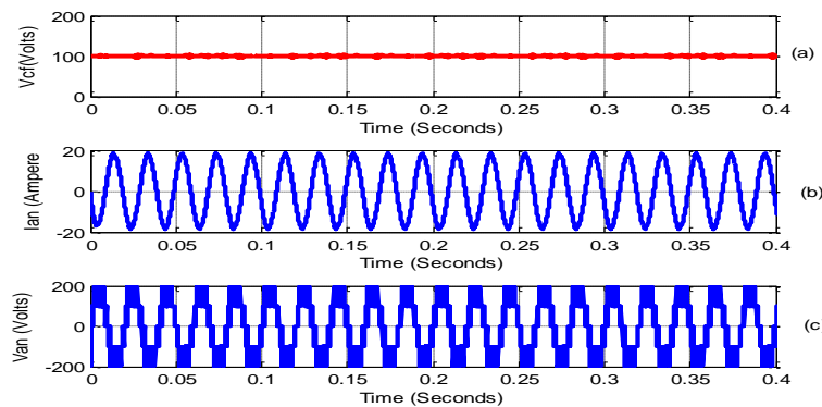
Fig. 22: (A) Capacitor voltage V_{cf} (C) Output Phase Current I_{an} (C) Output Phase Voltage V_{an} under natural capacitor voltage balancing operation for the Type B hybrid multi-level inverter of Figure 17 with per cycle switch state sequence of 1 \rightarrow 2 \rightarrow 3 \rightarrow 4 \rightarrow 5 \rightarrow 6 \rightarrow 7 \rightarrow 8 and C_f = 1500 \mu F , V_{dc} = 400 V , F_C = 5 kHz , F = 50 Hz , M = 0.8 , Z_L = (8+6j) \Omega with 100 V pre-charged capacitor voltage.
