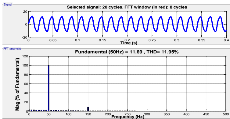
Fig. 13: Three Level Phase Current ( I_{an} ) With A Bypassed H-Bridge And Full Power.
