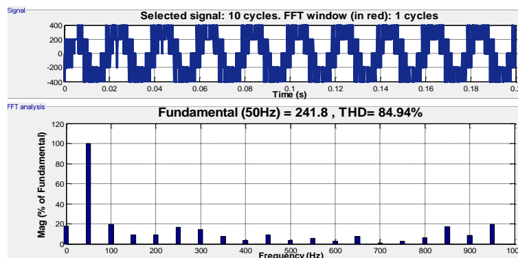
Fig. 26: Lines AB Voltage V_{AB} of five-level ANPC inverter of Figure 17 with A Shorted Capacitor. V_{dc} = 400V , F_c = 5 \text{ kHz} , F = 50\text{Hz} , M = 0.8 , Z_L = (8+6j) \Omega .
