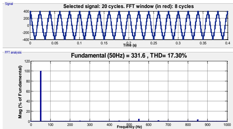
Fig. 11: Lines BC output Voltage ( V_{BC} ) with a balanced capacitor voltage for Type A hybrid multi-level inverter of Figure 1. V_{dc} = 400 V, F_C = 5 kHz, F_s = 50 Hz, M = 0.8 , Z_L = (8+6j) \Omega
