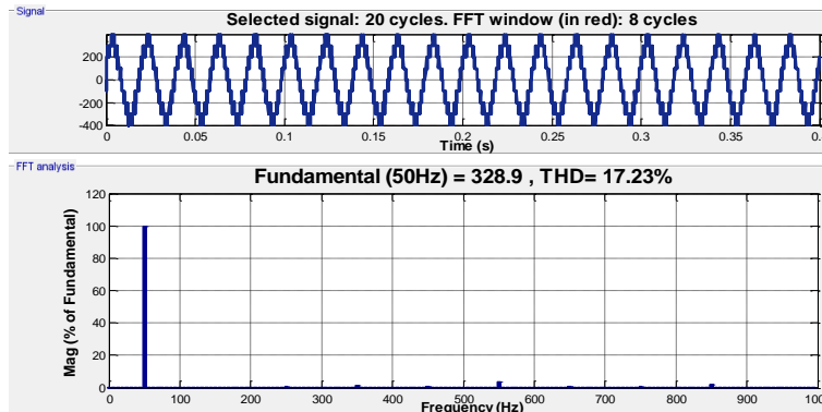
Fig. 12: Lines CA output Voltage ( V_{CA} ) with a balanced capacitor voltage for Type A hybrid multi-level inverter of Figure 1. V_{dc} = 400 V, F_C = 5 kHz, F_s = 50 Hz, M = 0.8 , Z_L = (8+6j) \Omega
