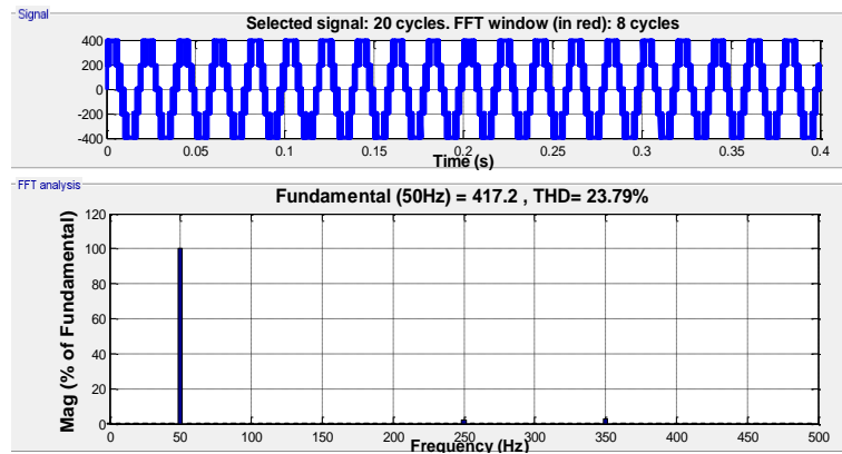
Fig. 15: Three Level Line-Line Voltage ( V_{AB} ) With A Bypassed H-Bridge And Full Power.
