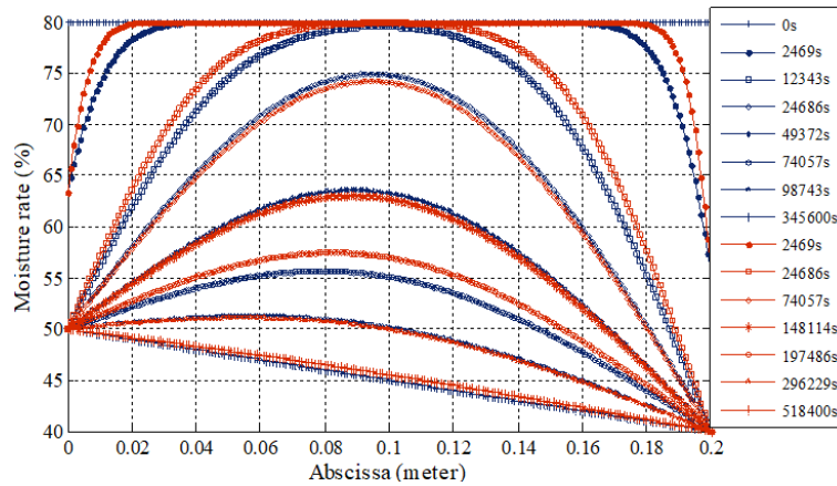
Fig. 3: Spatial Evolution of Moisture at Different Times of Simulation, for Different Pores Sizes: 0.003nm (Red Curves), 0.001nm (Blue Curves).
