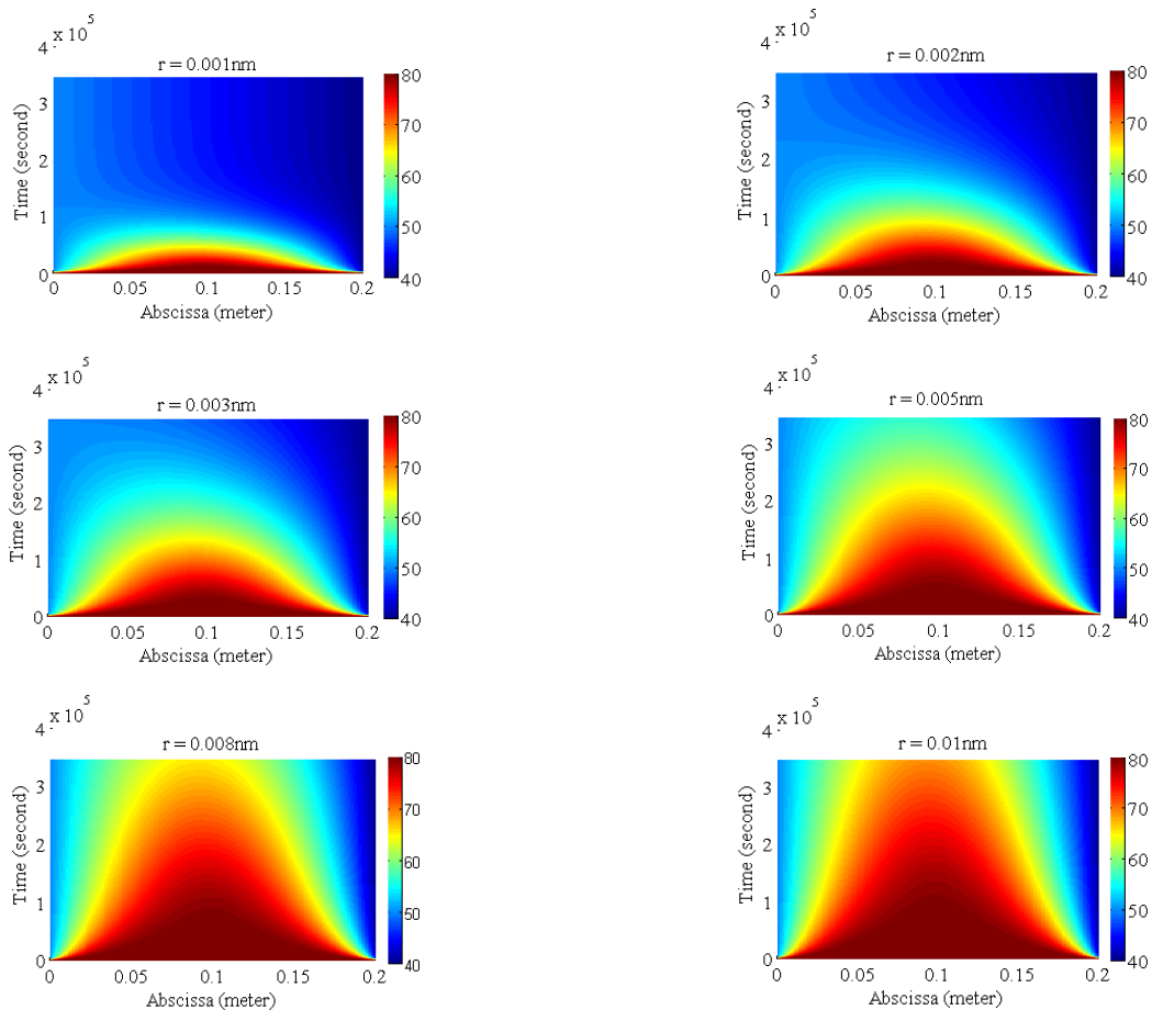
Fig. 2: Moisture Mapping for Different Pores Sizes.
