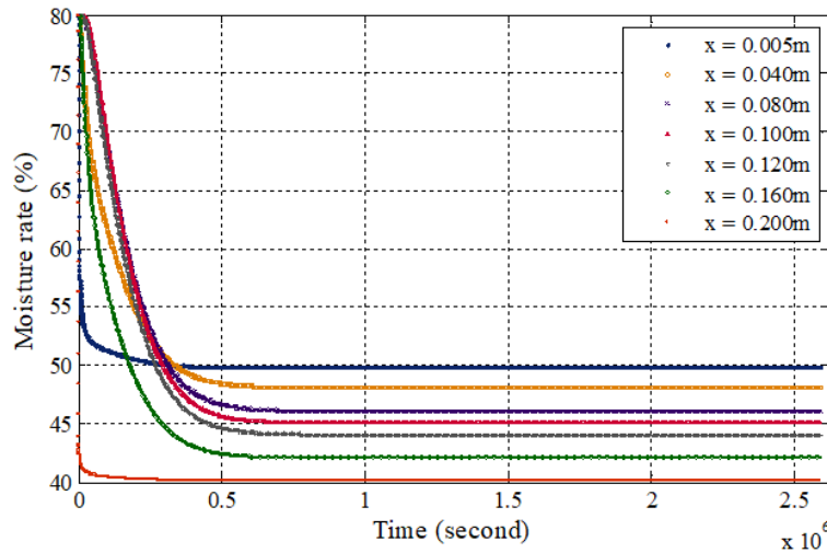
Fig. 4: Temporal Evolution of Moisture at Different Abscissa of the Wall for A Pore Radius of 0.001nm.
