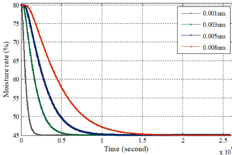
Fig. 5: Temporal Evolution of Moisture in the Middle of the Wall, for Different Pores Radius, 0.001nm (Black Curve), 0.003nm (Green Curve), 0.005nm (Blue Curve) and 0.008nm (Red Curve).
