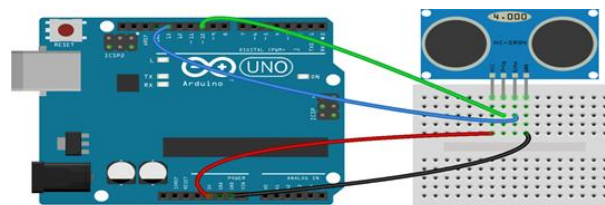
Fig. 1: Full Circuit Connection.
