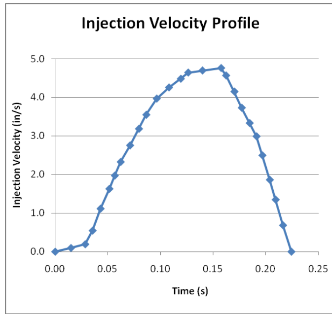
Fig. 8: Example of velocity profile from experimental data
