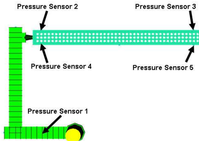
Fig. 4: Feed system, validation part, and sensor placement
