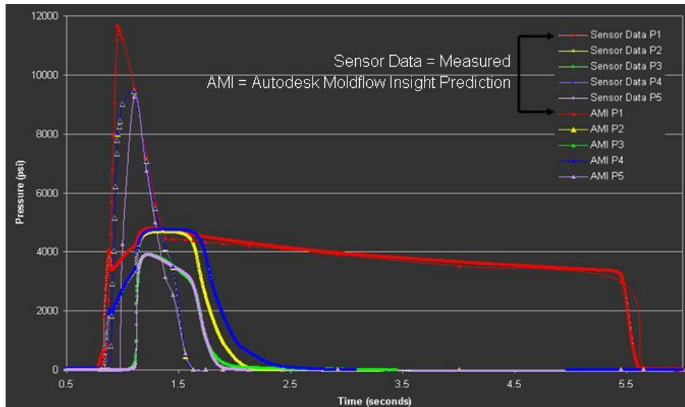
Fig. 5: Pressure profile output: Experiment versus Simulation using Ultramid A3EG7
